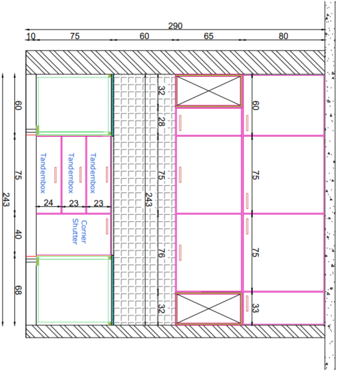
ELEVATION D
